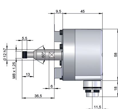
Drawing shaft type 1, anti-rotation system type 4, connection type 2
